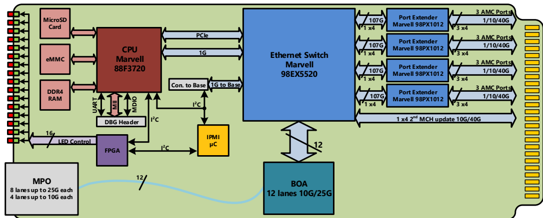
Figure 1 – Block Diagram NAT-MCH-HUB-E-40GX
