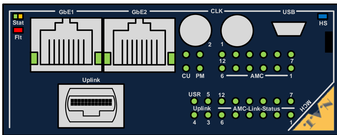
Figure 11 – NAT-MCH-HUB-E-40GX: Principle Drawing of Front Panel
