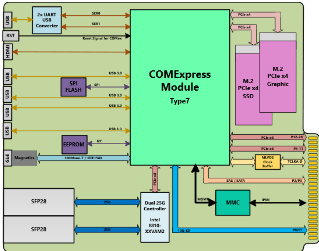
Figure 1 – Block Diagram NAT-AMC-CCT7
