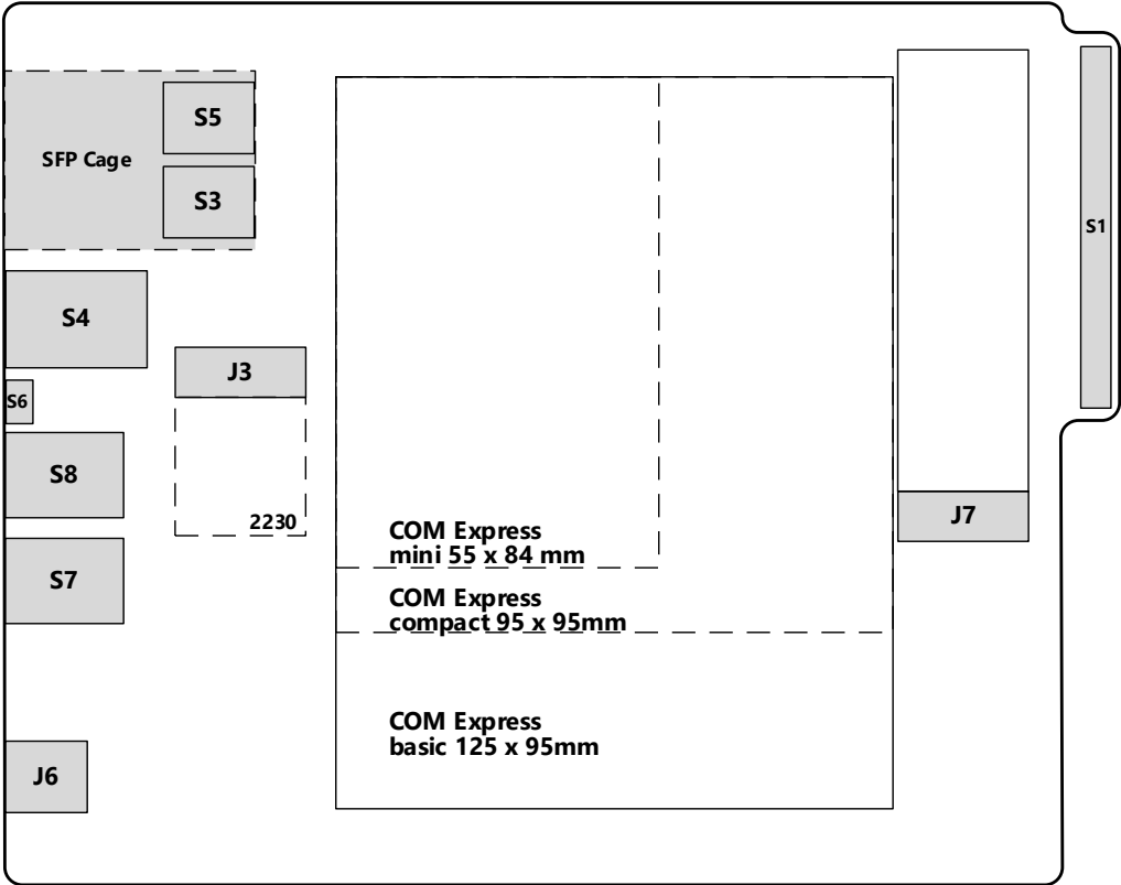
Figure 3 – NAT-AMC-CCT7 – Location Diagram – Top
