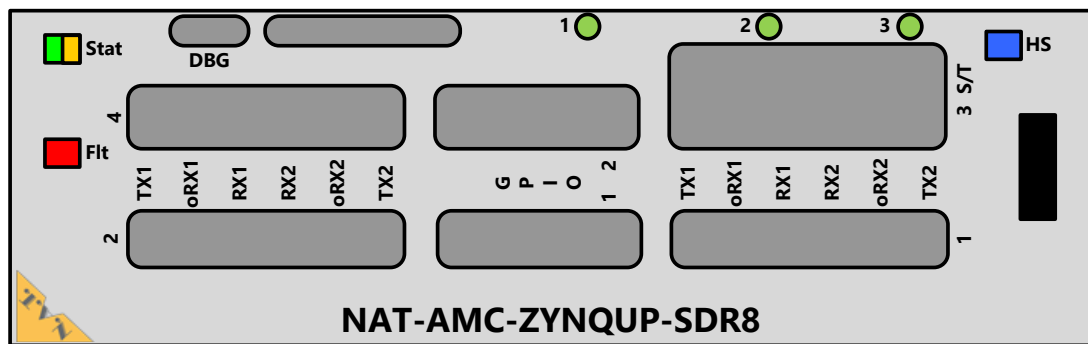
Figure 2 – Front Panel – Full Size
