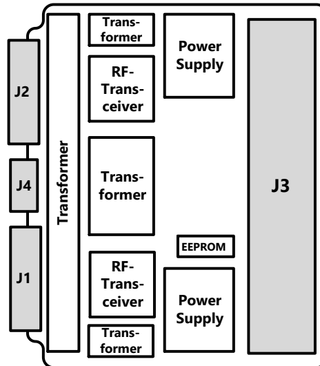
Figure 5 – NAT-FMC-SDR4-M Location Diagram – Top
