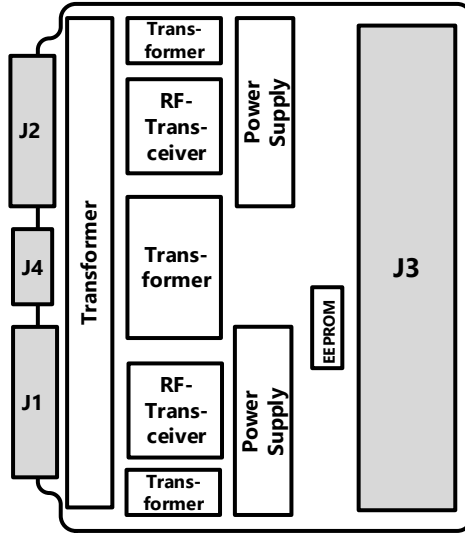
Figure 3 – NAT-FMC-SDR4-T Location Diagram – Top
