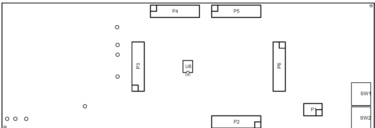
Figure 10: Piggy assembly drawing BOT side
