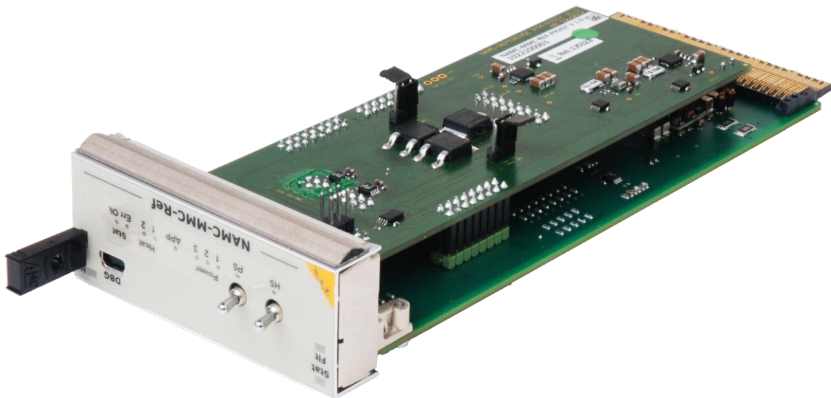
Figure 7: NAMC-MMC-REF with piggy board
