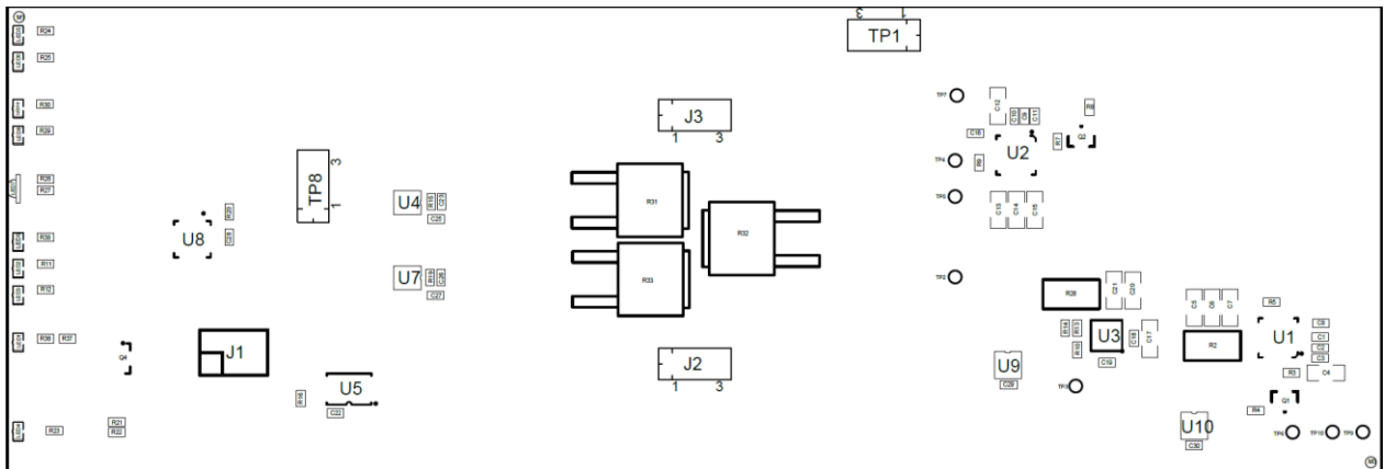
Figure 9: Piggy assembly drawing TOP side
