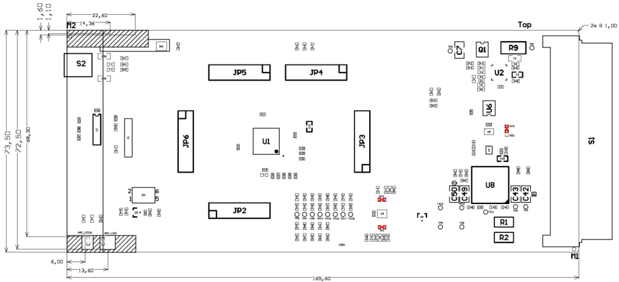
Figure 5: Connector and Switch Location – Overview
