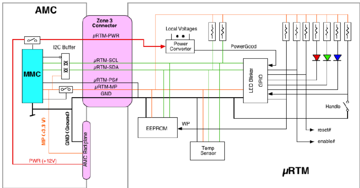
Figure 7: AMC/uRTM Management Block Diagram [6]
