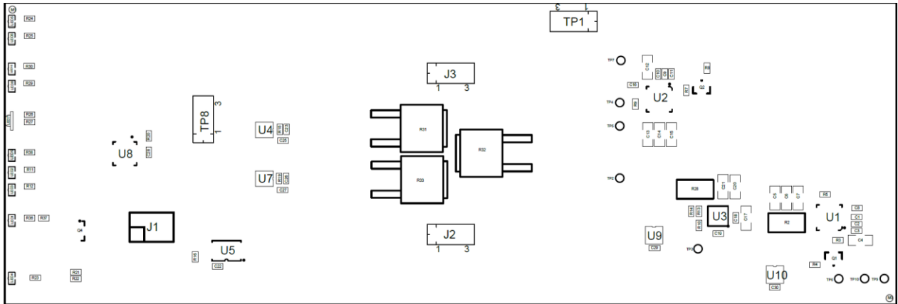
Figure 8: Piggy assembly drawing TOP side
