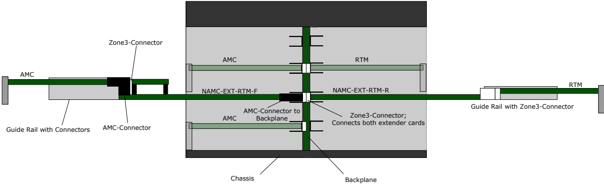
Figure 2: Mechanical Installation in a Chassis
