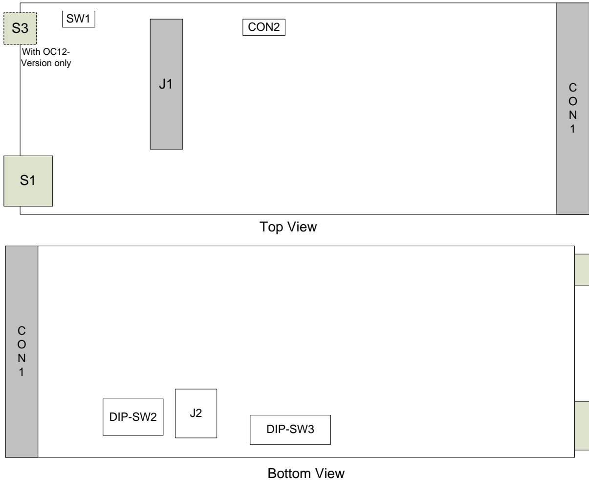
Figure 7: NAMC-8569-ATM – Connector and Switch Location Base Board – Overview
