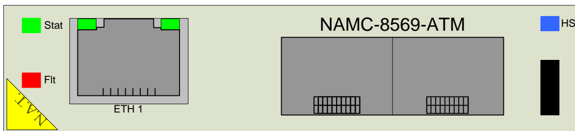
Figure 5: NAMC-8569-ATM – OC3-Version – Front Panel View
