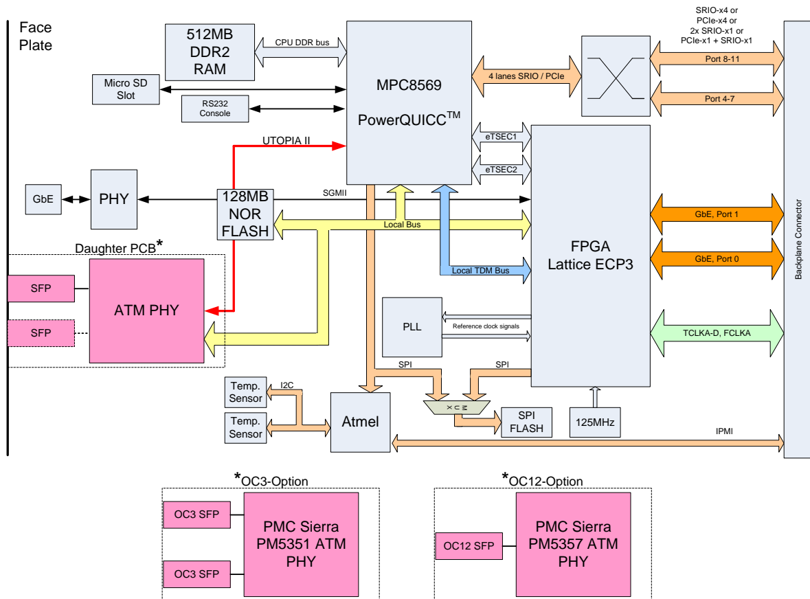
Figure 1: NAMC-8569-ATM – Block Diagram – Overview
