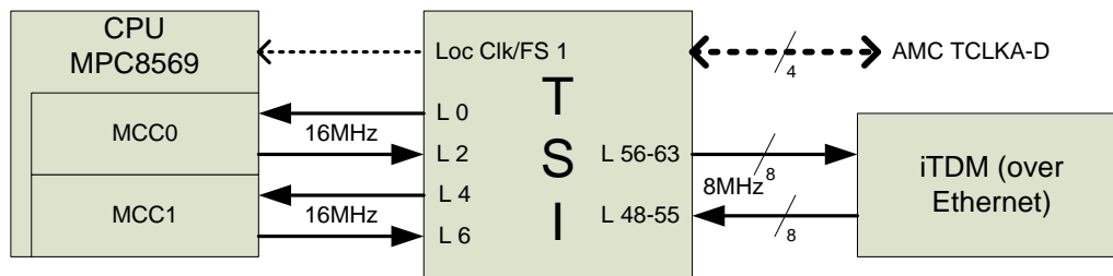
Figure 9: TDM Structure
